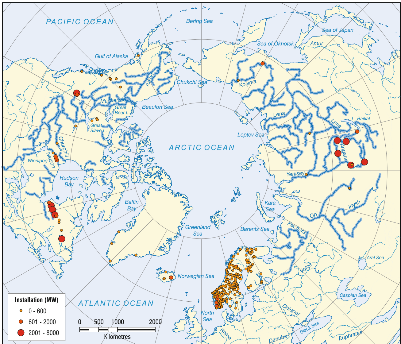
Fig. 4 Location and size of major hydroelectric facilities located in ice-dominated river regimes of the circumpolar North. All such stations will require major modifications to current operational regimes and possibly infrastructure modifications based on projected
