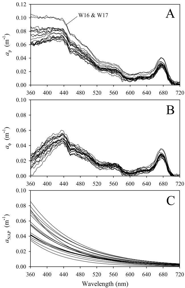
Figure 3. Particle absorption spectra at 10 m depth for the 18 stations sampled in Lake Taupo (values for the river station W15 are illustrated at Figure 4). (a) Total particle absorption, a_p , (b) phytoplankton absorption, a_\phi , and (c) nonalgal particles absorption a_{\text{NAP}} . For the three shallow stations located near the Tokaanu Tailrace, surface values are presented. Measured a_{\text{NAP}} was fitted to equation (5), excluding the 400–480 and 620–710 nm ranges to avoid the residual pigment absorption, and fitted spectra are presented in Figure 3c.
