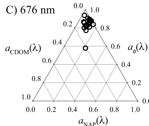
Figure 6. Ternary diagrams of the absorption budget for the 19 stations in Lake Taupo at (a) 380 nm, (b) 443 nm, and (c) 676 nm. The data point markedly different from the others corresponds to the river station W15. The three wavelengths were chosen to allow comparison with Figure 16 of Babin et al. [2003b]; 380 nm is a representative UV-A wavelength, 443 nm is in the blue region of the spectrum near the main absorption peak of phytoplankton, and 676 nm corresponds to the red absorption peak of CHLa.
