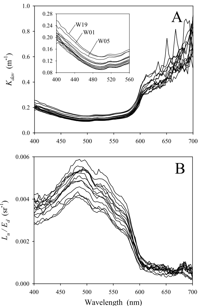
Figure 8. Apparent optical properties measured using an HyperPro radiometer. (a) Spectral attenuation coefficients for downwelling irradiance within the euphotic zone, K_{dav} ; (b) ratio of upwelling radiance to downwelling irradiance measured at \sim 0.1 m depth, L_u/E_d . The inset in Figure 8a shows detailed K_{dav}(400\text{--}560) .
