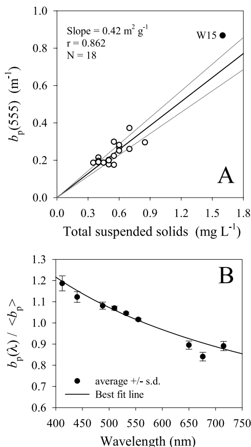
Figure 7. (a) Correlation between the particle scattering coefficient at 555 nm, b_p(555) , and total suspended solids (TSS); (b) spectral variation in b_p illustrated by the average spectra ( \pm 1 standard deviation) of the b_p(\lambda)/\langle b_p \rangle ratio, where \langle b_p \rangle is the spectrally averaged scattering coefficient of particles. The river station W15 was excluded from the regression in Figure 7a and was not included in the average spectra presented in Figure 7b.
