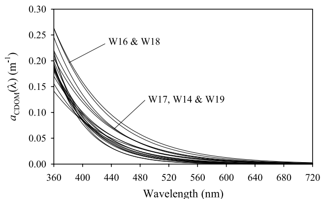
Figure 5. Absorption spectra of CDOM ( a_{\text{CDOM}} ) for the 18 stations sampled in Lake Taupo. In absence of direct measurement, a_{\text{CDOM}} was estimated as the difference between a_{\text{AC-9}} and a_p fitted to the exponential model of equation (8) (see section 2.3).
