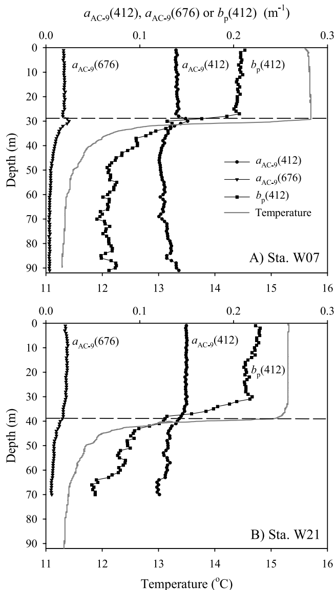
Figure 2. Vertical profiles of temperature, absorption coefficients at 412 nm and 676 nm, and scattering coefficient at 412 nm as measured using a WETLabs AC-9 at (a) Whangamata Bay (W07) and (b) at a center lake station (W21). Depth is 100 and 154 m at stations W07 and W21, respectively, and the mixed layer depth was 29 and 39 m at stations W07 and W21, respectively (as shown by a dashed line).
