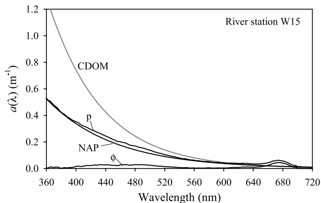
Figure 4. Absorption spectra of CDOM ( a_{\text{CDOM}} ), total particles ( a_p ), phytoplankton ( a_\phi ) and nonalgal particles ( a_{\text{NAP}} ) at the river station W15.
