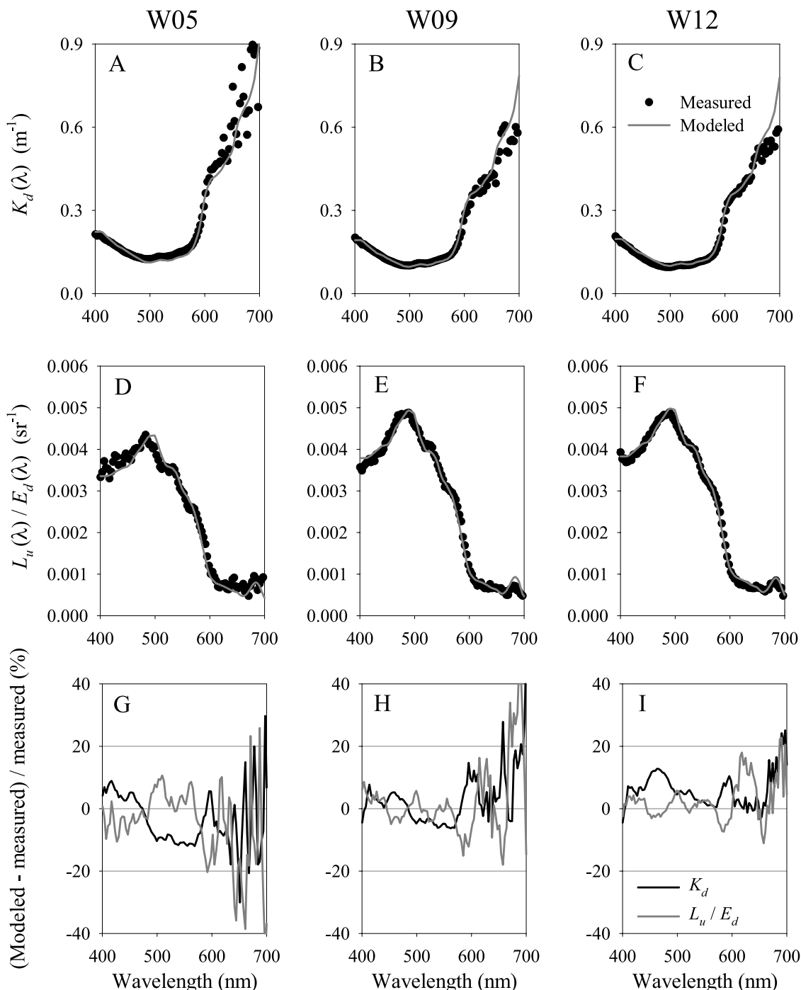
Figure 9. Measured and modeled K_d(\lambda) and L_u(\lambda)/E_d(\lambda) and the percent difference between modeled and measured values at three stations representing extremes in K_d , CHL a concentration, and atmospheric conditions. (a, d, and g) Station W05 at 16h00, clear sky, b_{bp}/b_p = 0.008 . (b, e, and h) Station W09 at 13h00, overcast b_{bp}/b_p = 0.010 . (c, f, and i) Station W12 at 13h00, overcast, b_{bp}/b_p = 0.012 . See color version of this figure at back of this issue.
